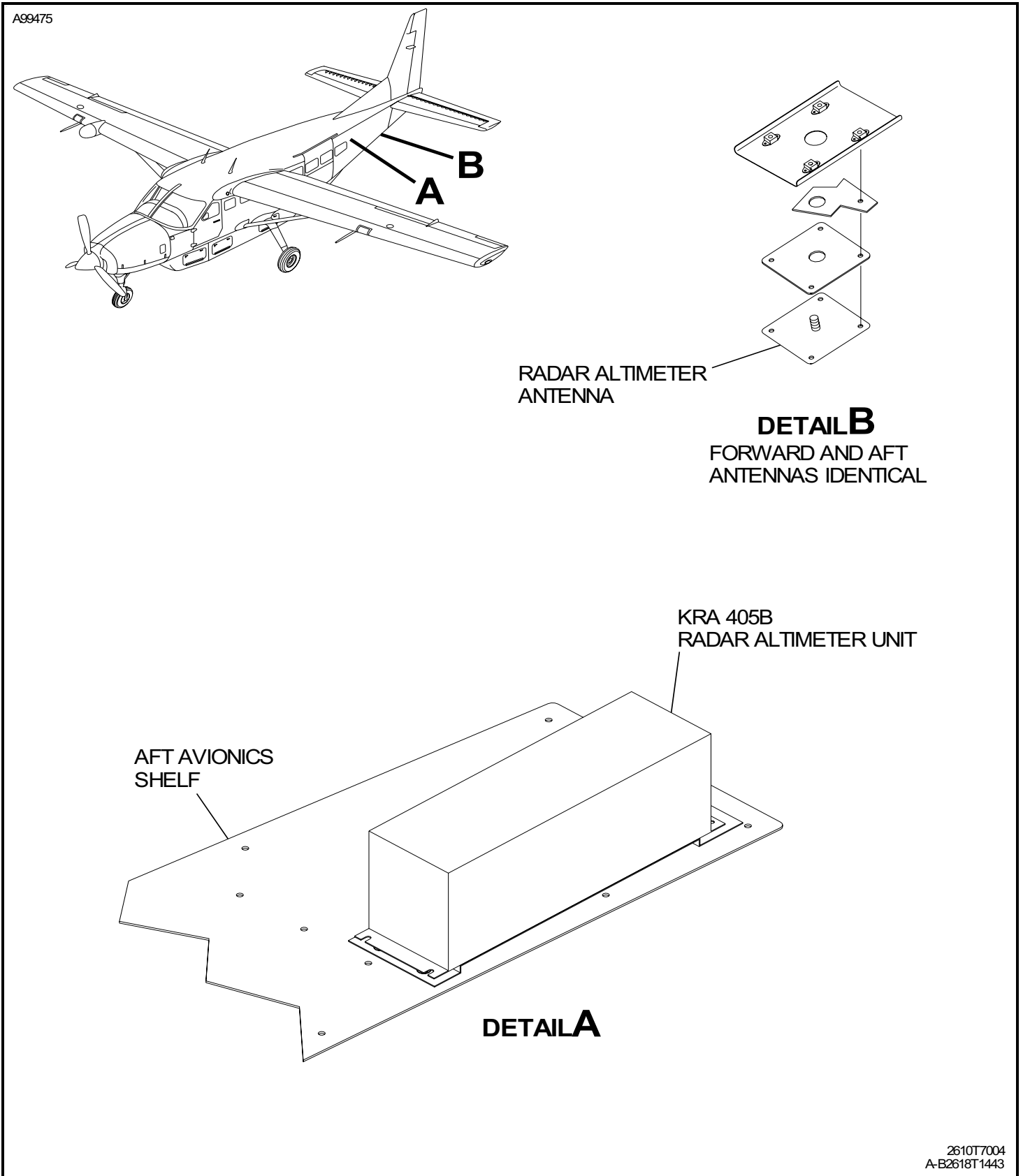
Figure 1 : Sheet 1 : Bendix/King KRA 405B Radio Altimeter System
